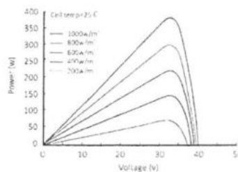
Power-Voltage Curve (LR4-60HPH-365M)
