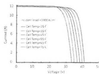
Current-Voltage Curve (LR4-60HPH-365M)
